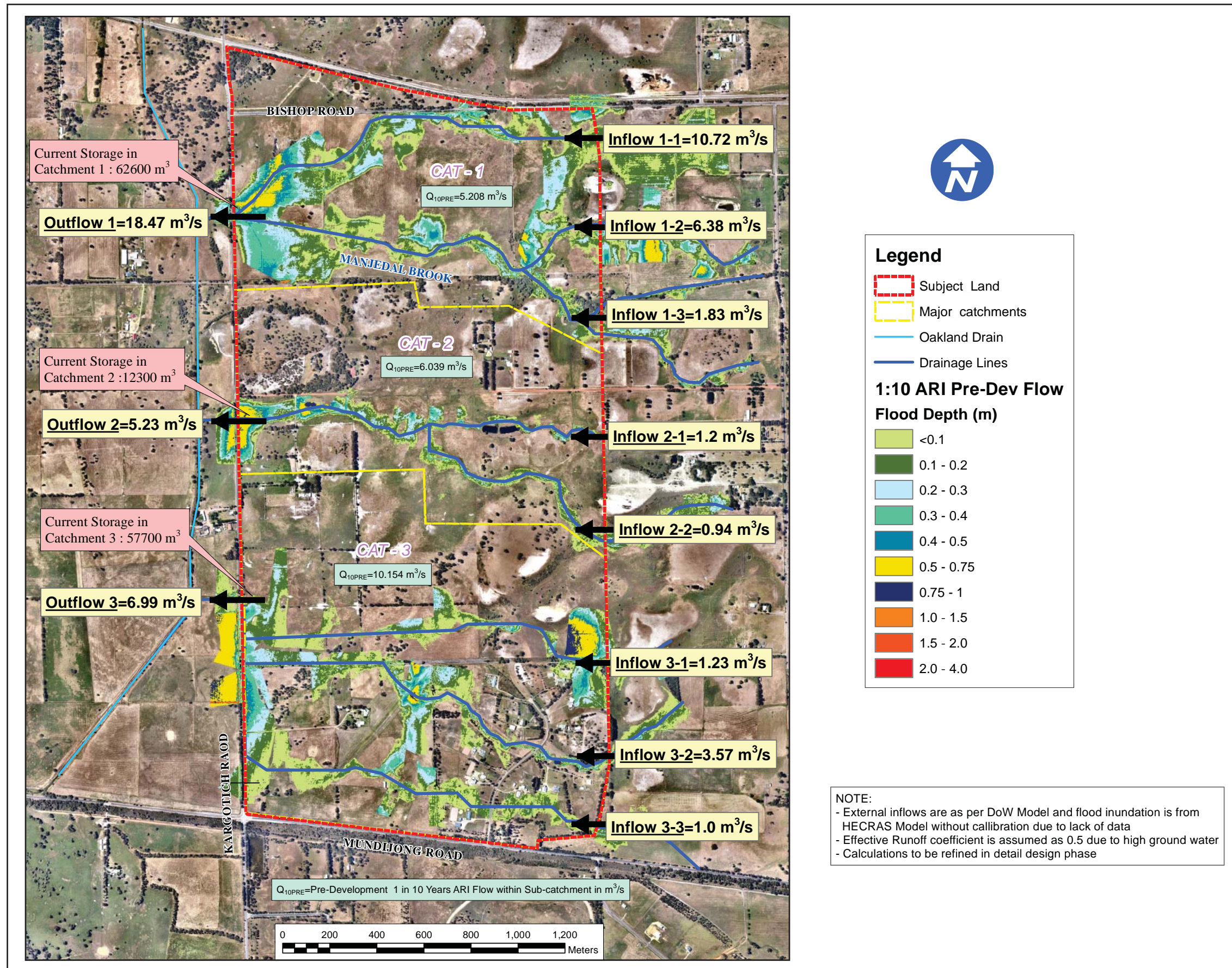
Figure 7 - 1 in 10 Years ARI Pre-Development Flows
