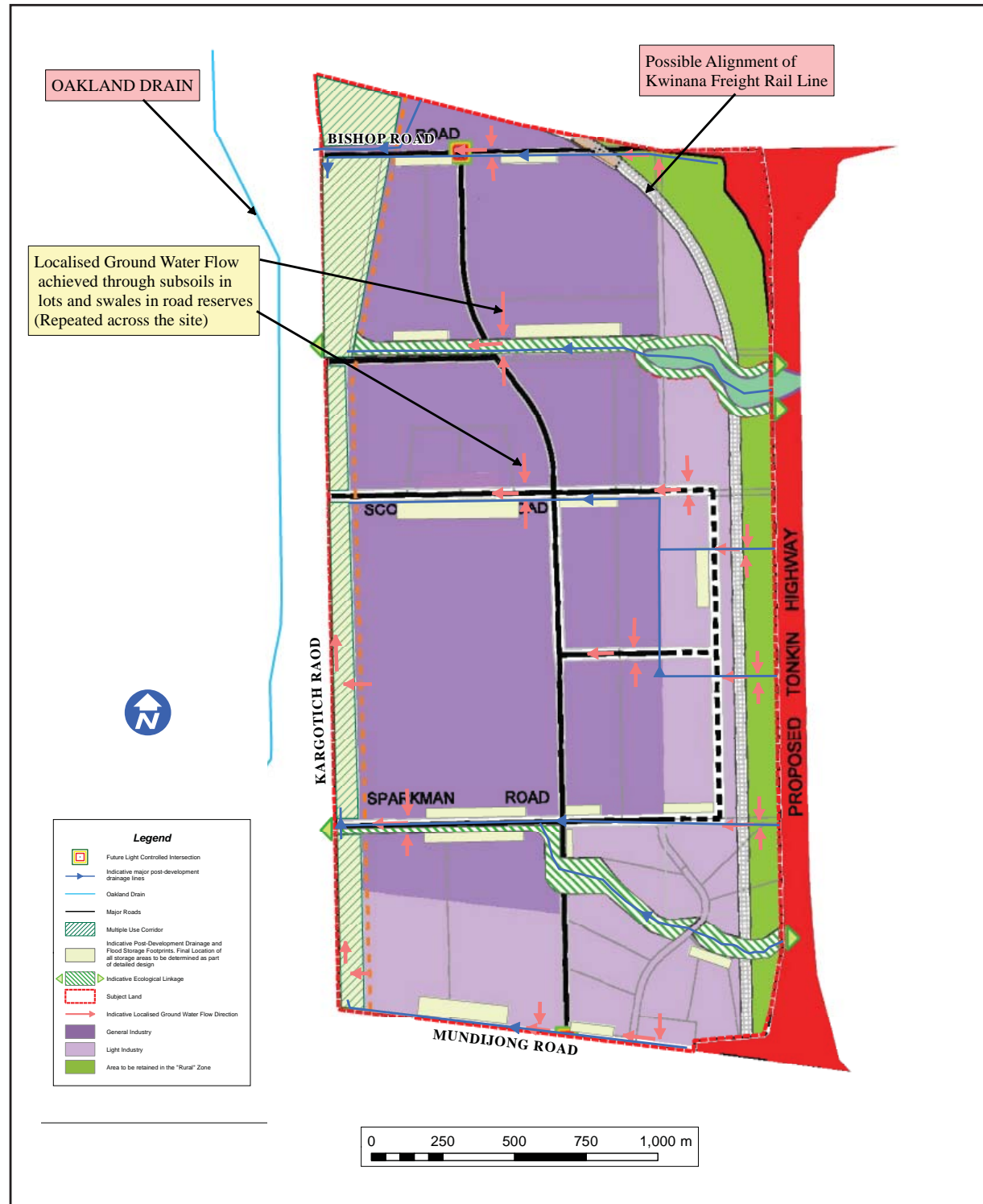
Figure 16- Post Development Ground water Management Plan
