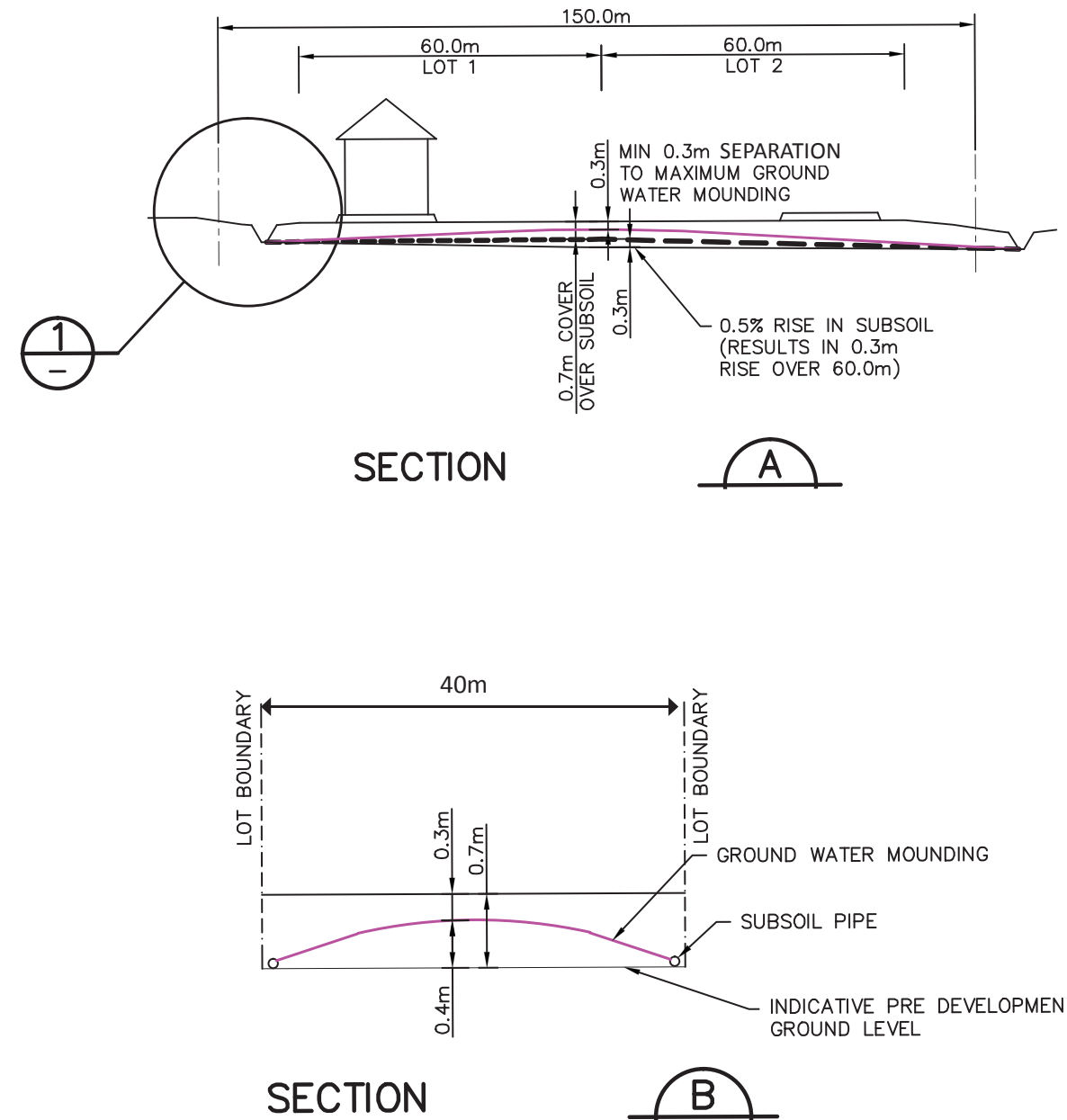
Figure 18a - Typical Lot Ground Water Management
