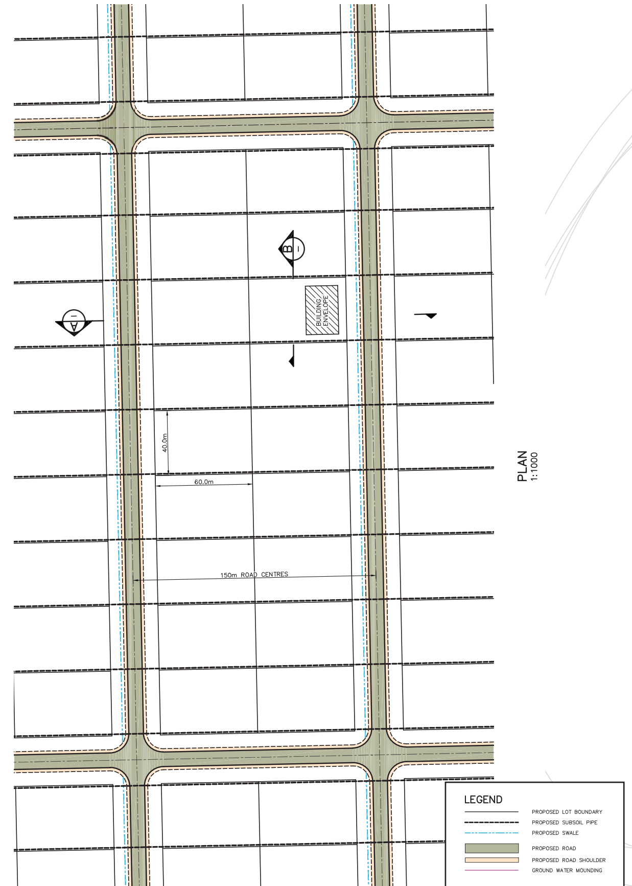
Figure 17- Typical Subsoil and Drainage Layout Plan
