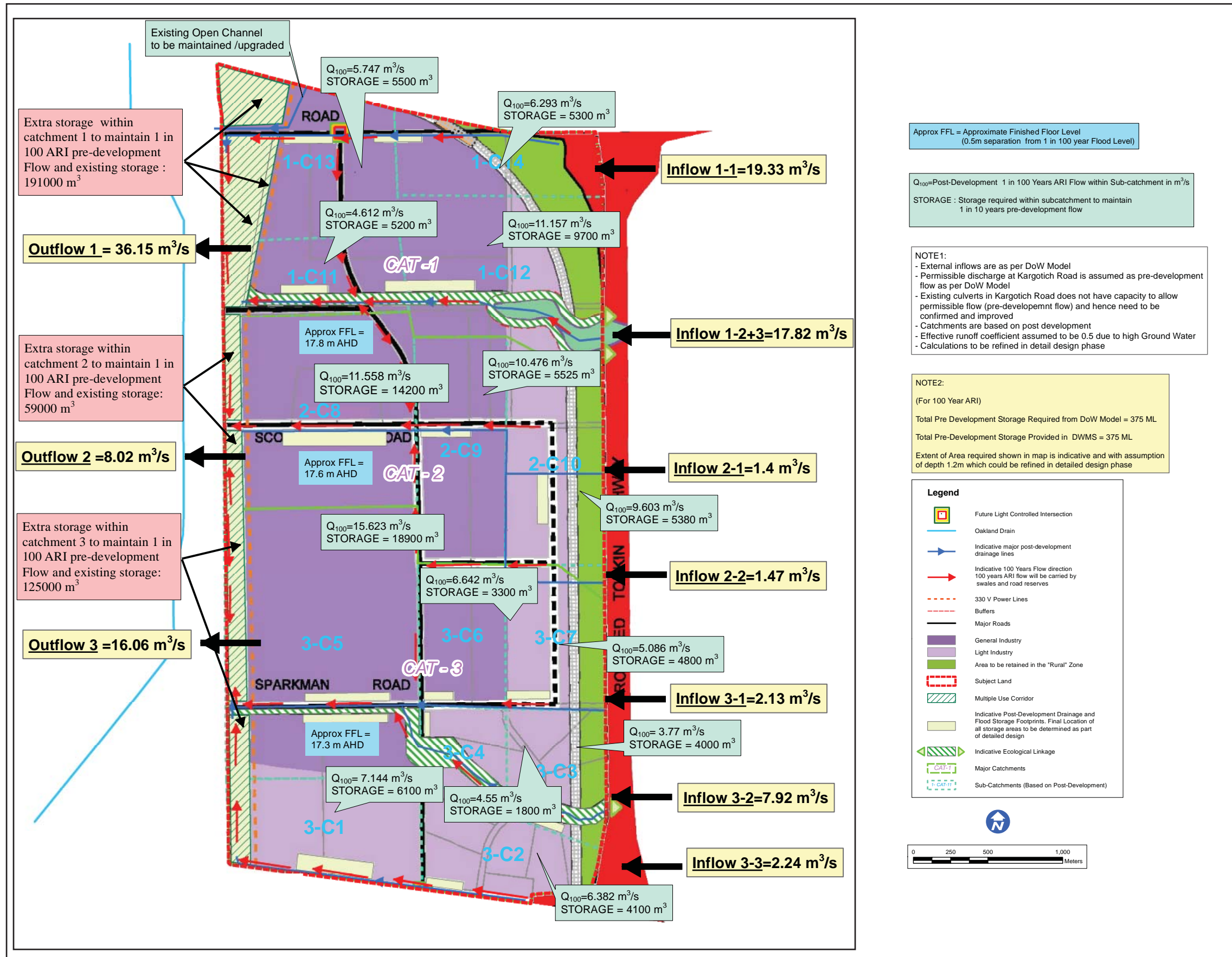
Figure 12 - 1 in 100 year Post Development Drainage Plan
