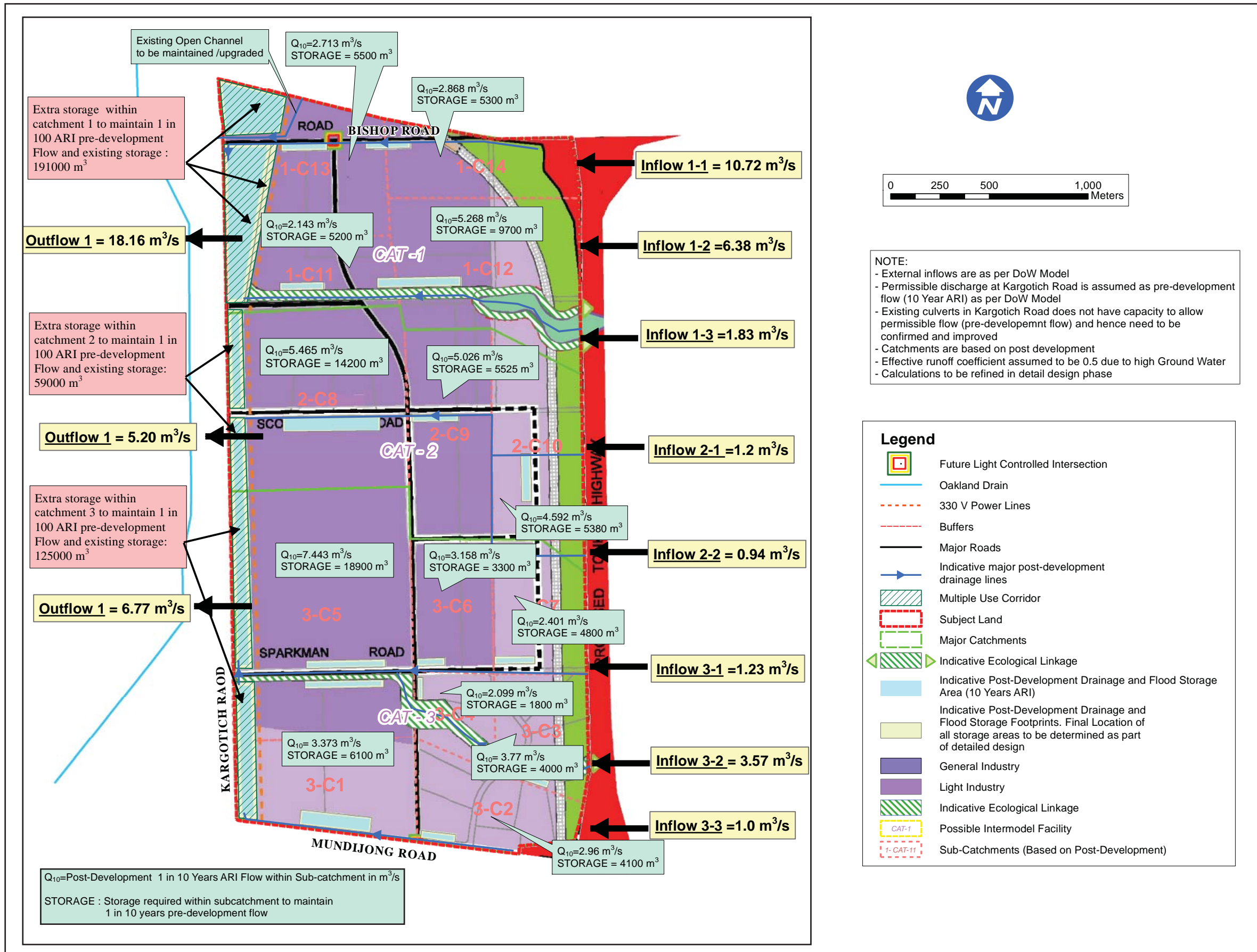
Figure 11 - 1 in 10 year Post Development Drainage Plan
