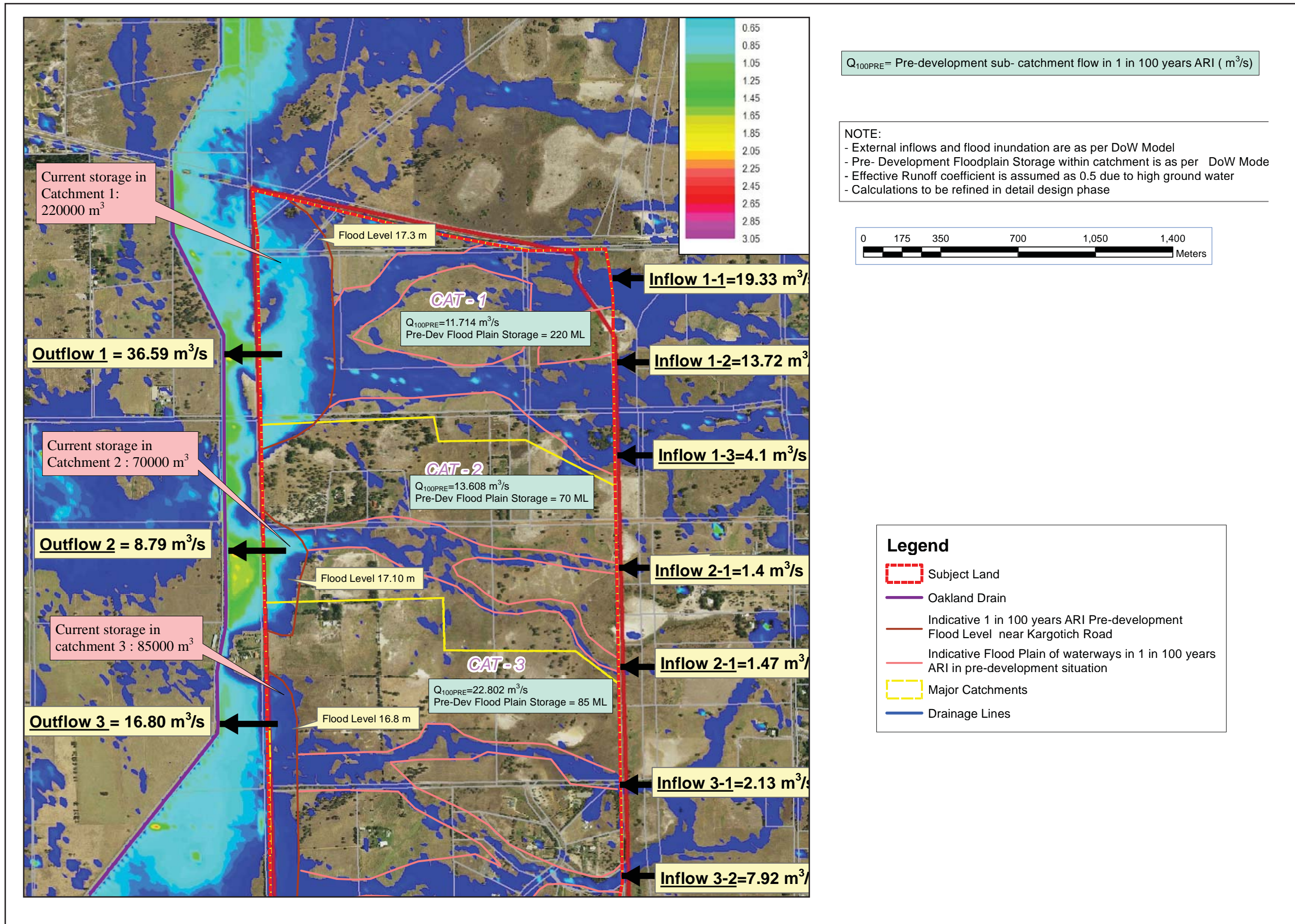
Figure 8 - 1 in 100 Years ARI Pre-Development Flows
