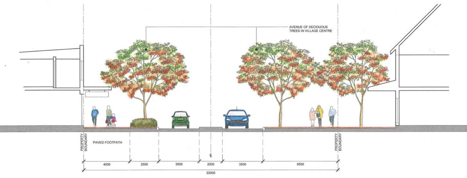
C SECTION C : MEAD STREET EXTENSION 1:100 @ A3
