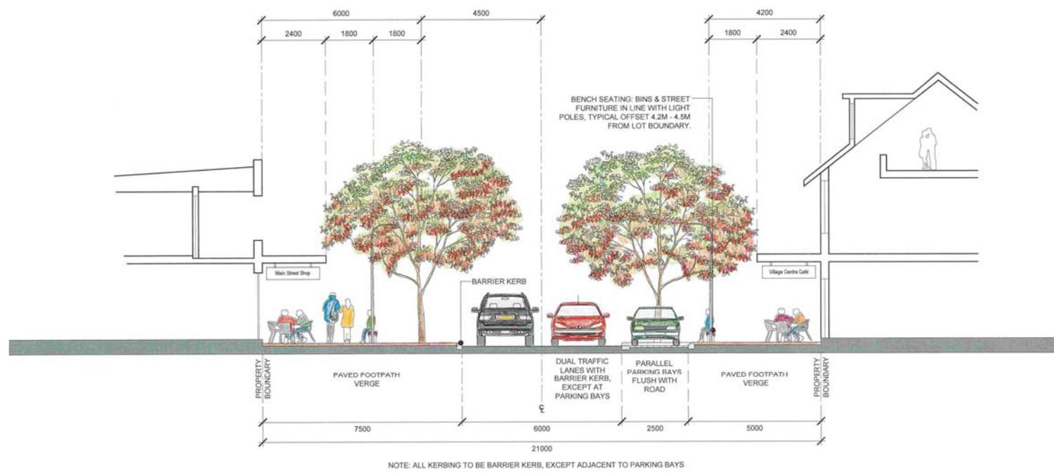
A SECTION A : MAIN STREET 1:100 @ A3
