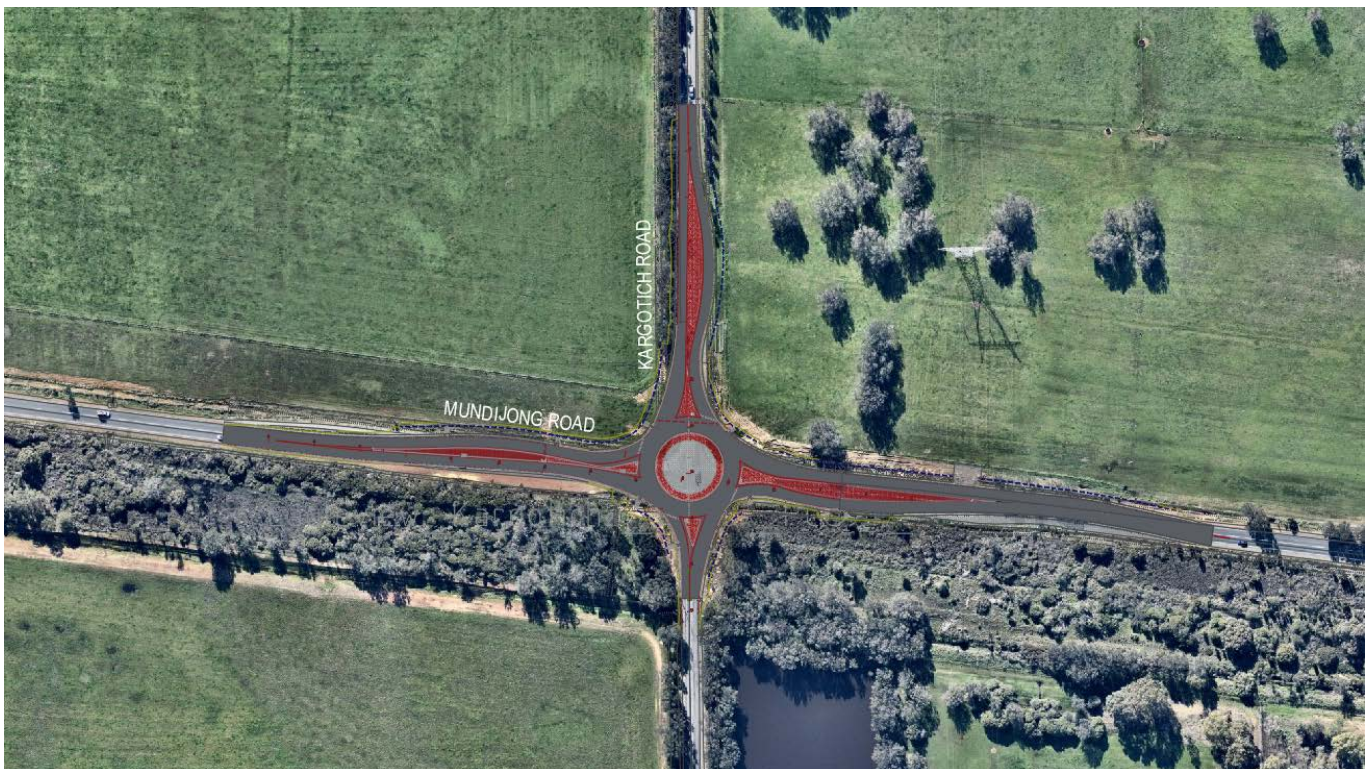
Figure 1: Proposed Mundijong Road/Kargotich Road Roundabout
